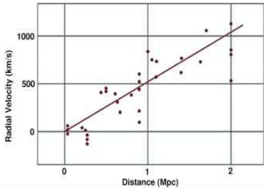
Hubbles' Original Data
