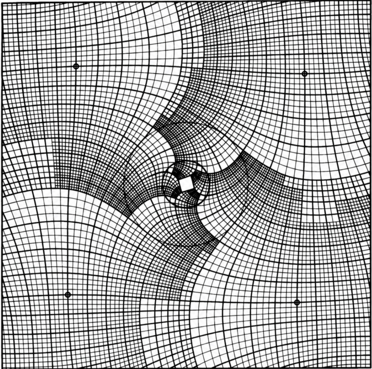
Figure 2. A reconstruction of Escher's expanding grid. After one complete circuit around the centre, the grid returns to the same orientation at 256 times its original scale. Equivalently, each quarter-turn changes the scale by a factor of four, since 4^4=256 . Redrawn after Escher's original study, adapted from a figure in [3].
