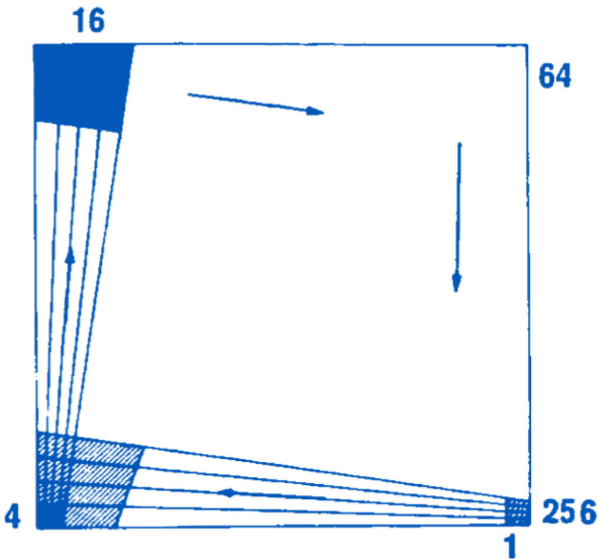
Figure 1. Cyclic expansion with fourfold magnification around a loop. Each successive stage increases the scale by a factor of 4, giving a cumulative magnification of 44 = 256 after one complete circuit. Based on figures in [3].
